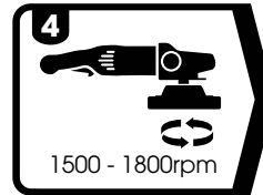
4 Spread and compound at 1500 - 1800rpm. Apply more water if necessary
